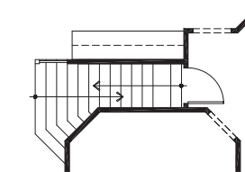
Stair @ Opt. Second Floor
