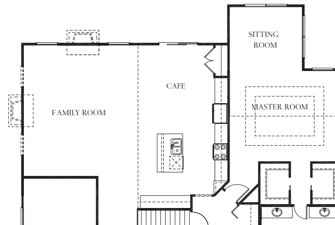
Ext. Family & Sitting Rooms
