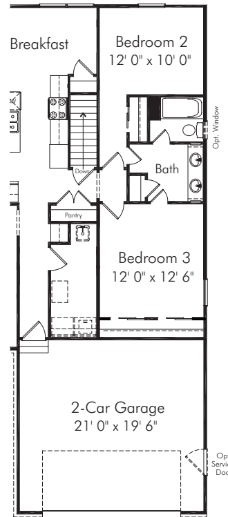
Optional Shared Bath Plan @ Eastern Seaboard and Farmhouse Elevations
