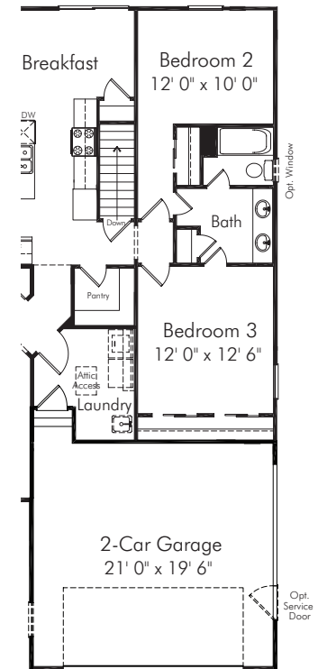
Optional Shared Bath Plan @ Craftsman, Cottage, Arts & Crafts, and Bungalow Elevations
