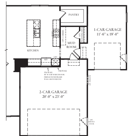
Partial First Floor at Opt. 1-car Garage w/ 2-Car Front Load Garage
