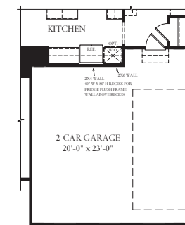
Partial First Floor at Opt. 2-Car Side Load Garage
