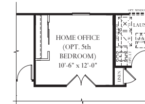
Partial Second Floor Plan at Opt. Home Office
