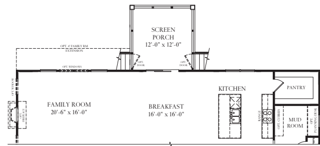
Partial First Floor at Opt. Screen Porch
