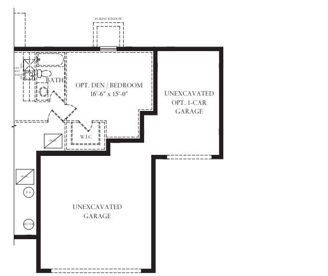
Partial Lower Level at Opt. 1-Car Garage w/ 2-car Front Load Garage
