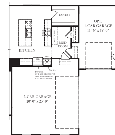
Partial First Floor at Opt. 1-car Garage w/ 2-Car Side Load Garage
