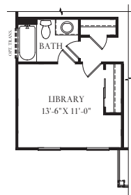
Partial First Floor plan at Library - Federal
