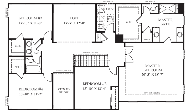
Partial Second Floor Plan w/ Opt. Bath #3 @ Craftsman Elevation
