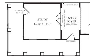
Partial First Floor at Opt. Wrap Around Porch - Craftsman
