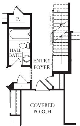
Opt. Partial First Floor Plan @ Opt. Slab on Grade
